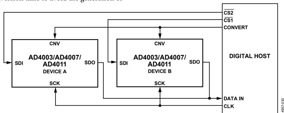
Figure 61. \overline{\text{CS}} Mode, 4-Wire Without Busy Indicator Connection Diagram
