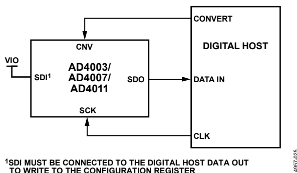
Figure 55. \overline{\text{CS}} Mode, 3-Wire Without Busy Indicator Connection Diagram
