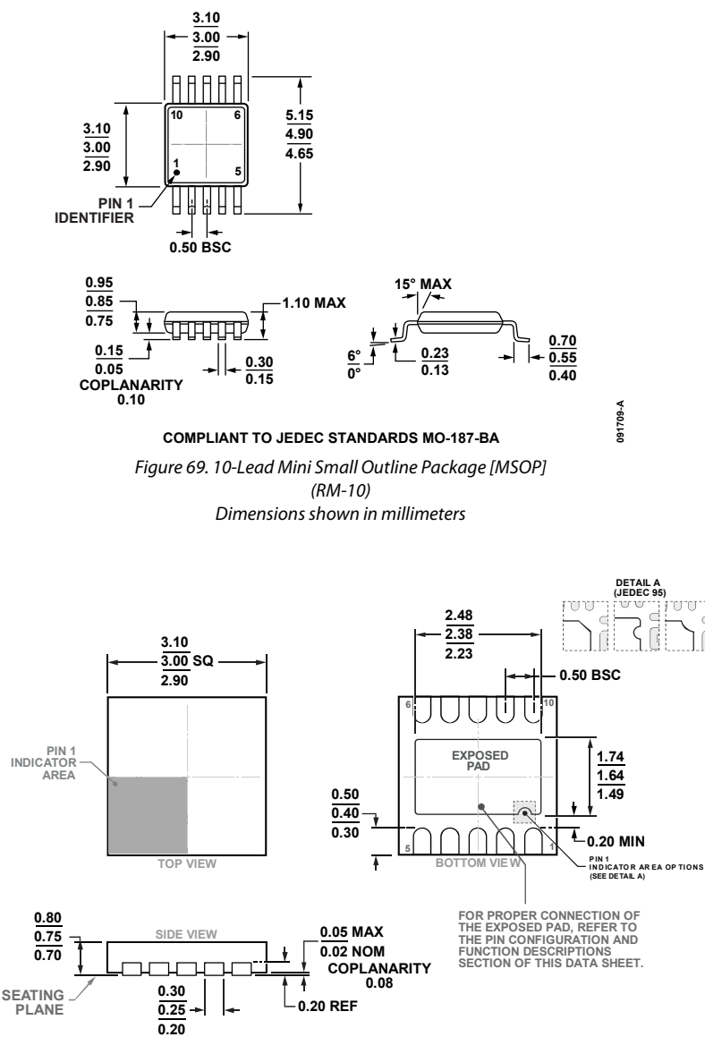
Figure 70. 10-Lead Lead Frame Chip Scale Package [LFCSP] 3 mm x 3 mm Body and 0.75 mm Package Height (CP-10-9)
