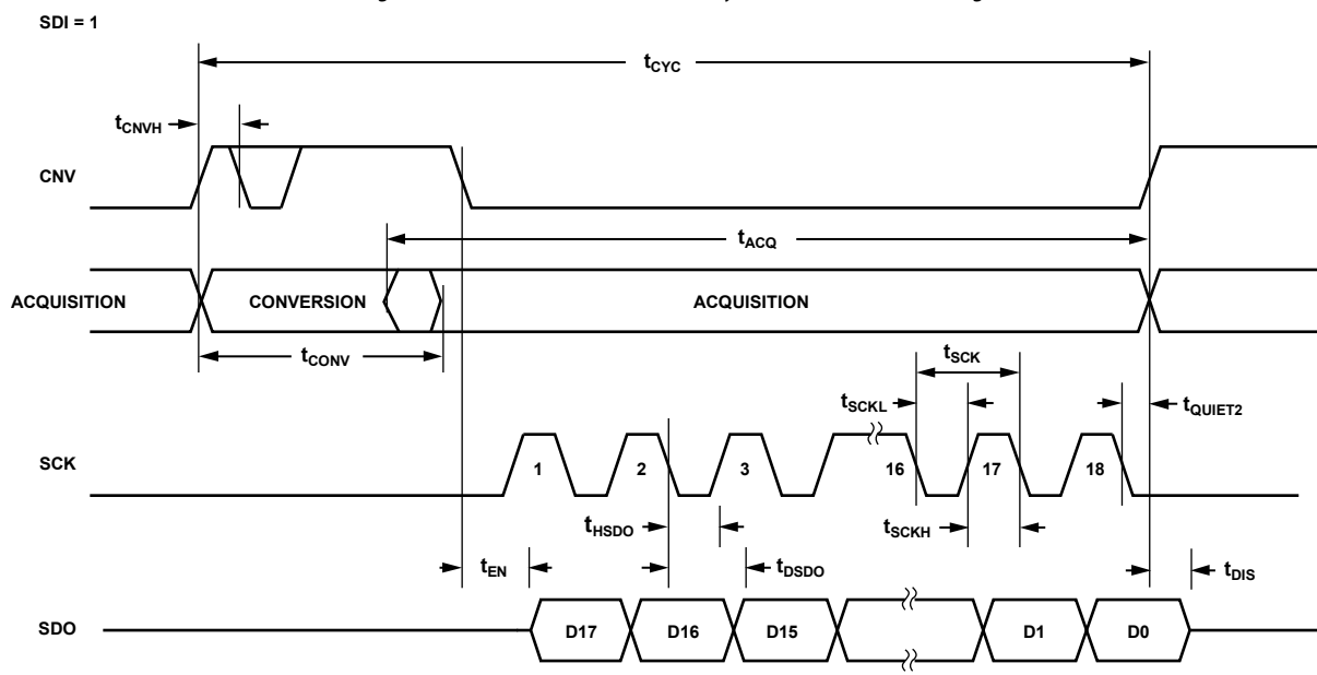
Figure 56. \overline{\text{CS}} Mode, 3-Wire Without Busy Indicator Serial Interface Timing Diagram (Status Bits Not Shown)
