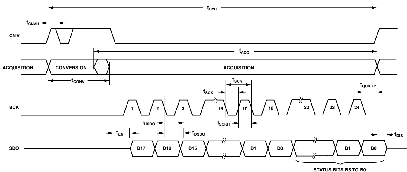
Figure 52. \overline{\text{CS}} Mode, 3-Wire Without Busy Indicator Serial Interface Timing Diagram Including Status Bits
