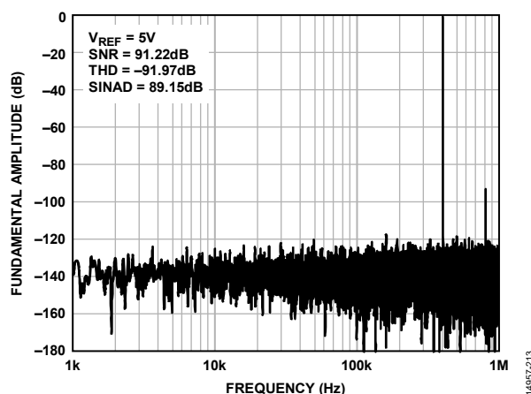
Figure 16. 400 kHz, -0.5\text{ dBFS} Input Tone FFT
