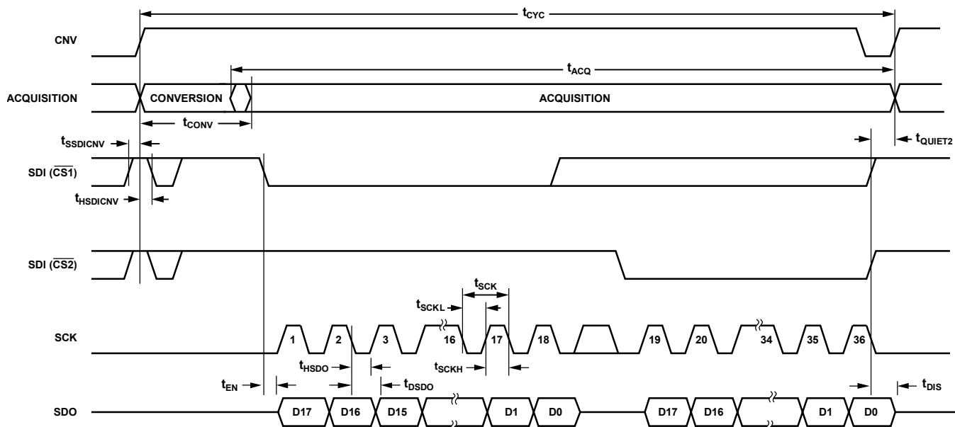
Figure 62. \overline{\text{CS}} Mode, 4-Wire Without the Busy Indicator Serial Interface Timing Diagram (Status Bits Not Shown)
