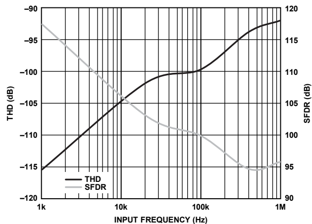
Figure 20. THD and SFDR vs. Input Frequency
