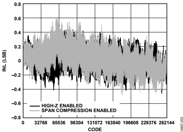
Figure 7. INL vs. Code for High-Z and Span Compression Modes Enabled, V_{REF} = 5\text{ V}
