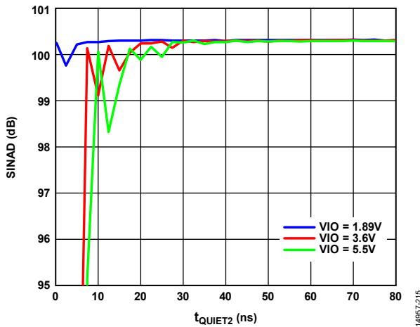
Figure 24. SINAD vs. t_{\text{QUIET2}}
