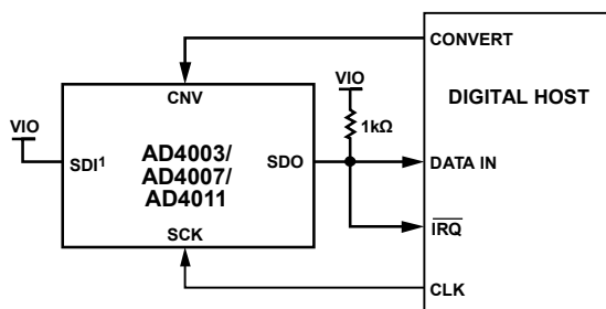
Figure 57. CS Mode, 3-Wire with Busy Indicator Connection Diagram
