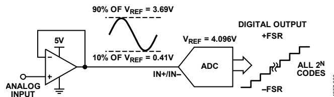
Figure 46. Span Compression
