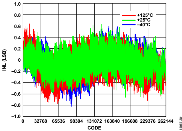
Figure 6. INL vs. Code for Various Temperatures, V_{REF} = 2.5\text{ V}
