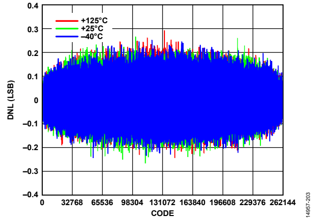
Figure 8. DNL vs. Code for Various Temperatures, V_{REF} = 5\text{ V}
