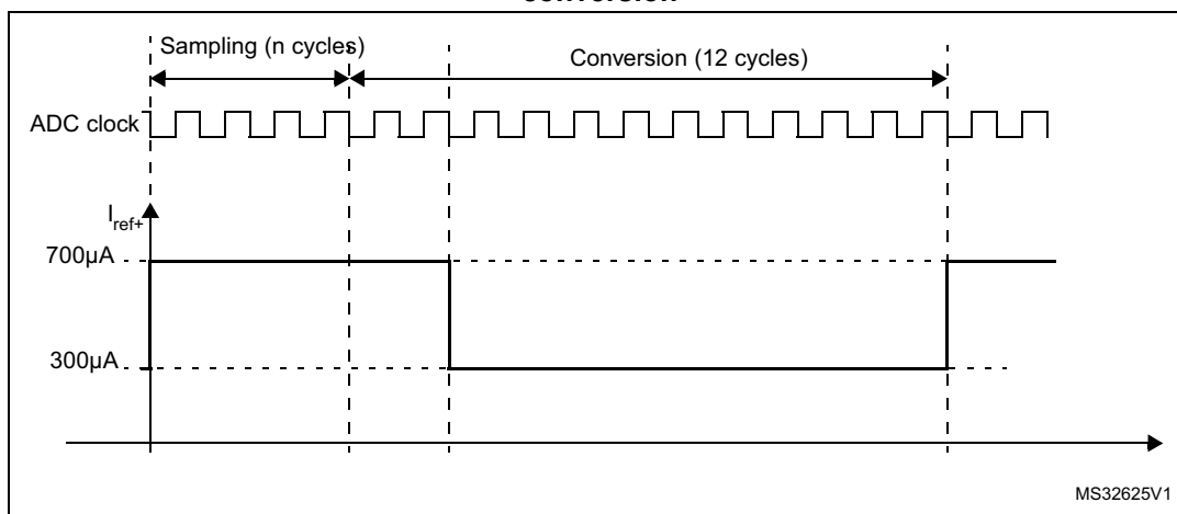
Figure 40. Maximum dynamic current consumption on V_{REF+} supply pin during ADC conversion
