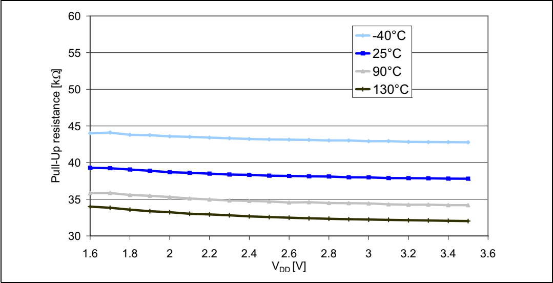
Figure 23. Typical pull-up resistance R_{PU} vs V_{DD} with V_{IN}=V_{SS}
