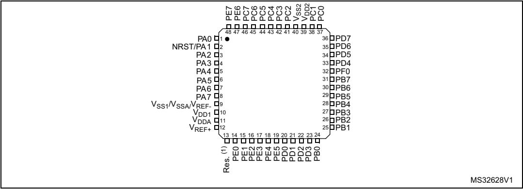
Figure 3. STM8L151Cx 48-pin pinout (without LCD)
