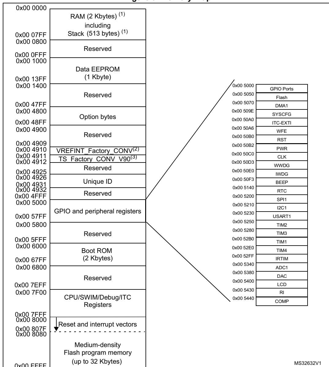
Figure 9. Memory map
