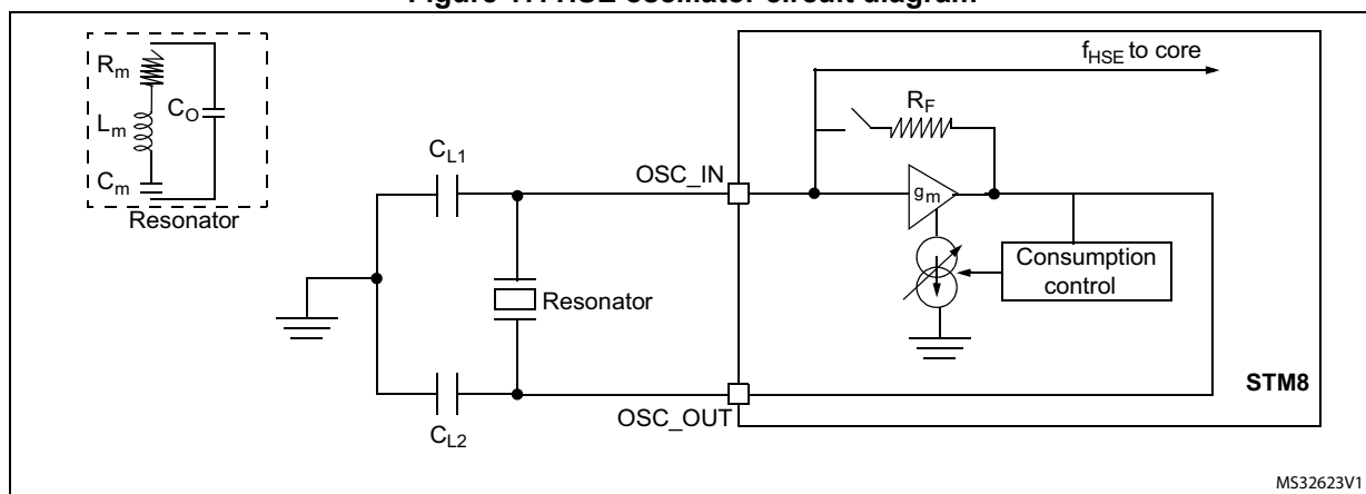
Figure 17. HSE oscillator circuit diagram
