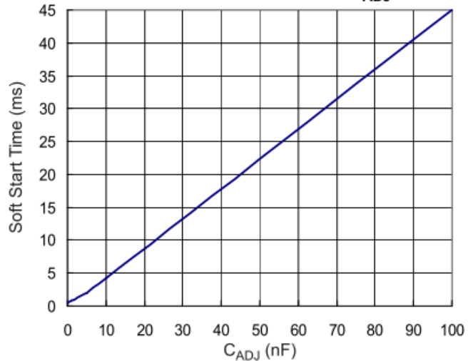
Soft Start Time vs. C_{ADJ}
