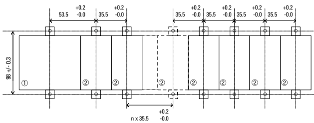
Mounting Hole Layout (Using Mounting Slides)
