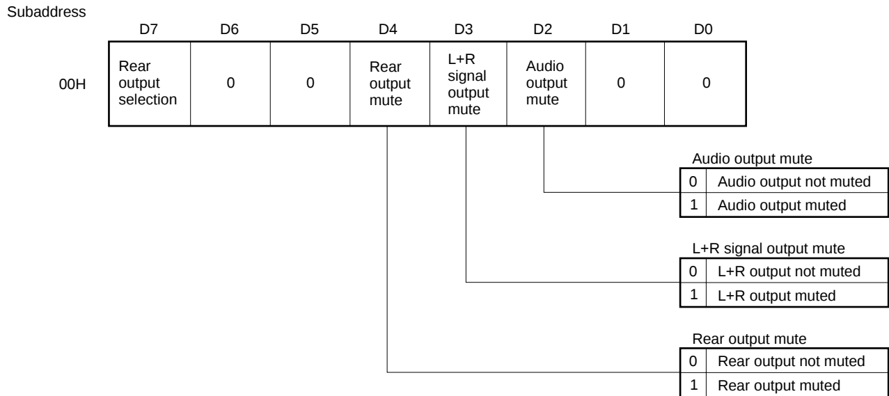
Fig. 4-13 Mute ( \mu PC1853-02)
