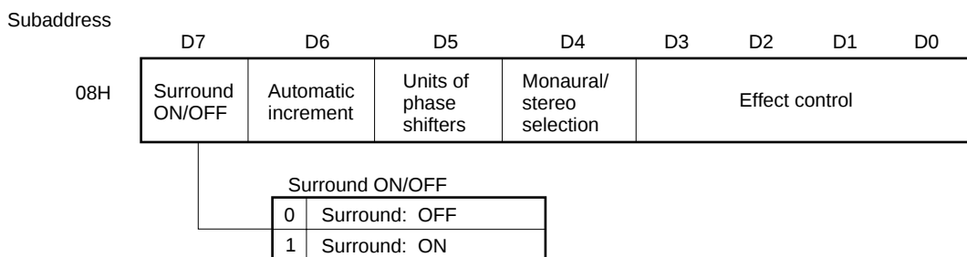
Fig. 4-12 Surround ON/OFF
