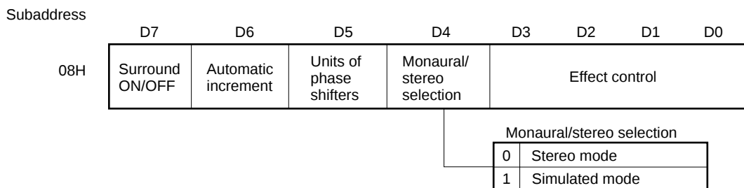
Fig. 4-10 Monaural/Stereo Selection
