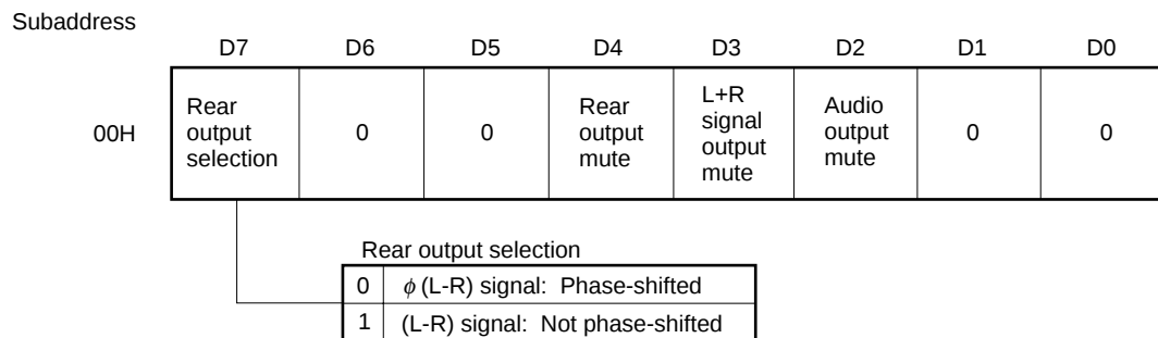
Fig. 4-14 Rear Output Selection ( \mu PC1853-02)
