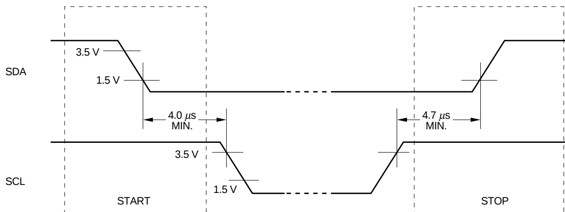
Fig. 3-2 Start/Stop Condition of Data Transfer
