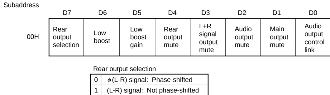
Fig. 4-4 Rear Output Selection ( \mu PC1853-01)
