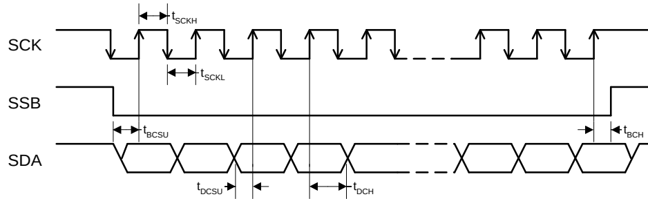
FIGURE 11. Data Interface Timing(SPI)
