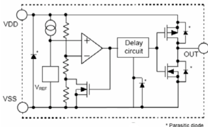
CMOS OUTPUT (EC9519C)
