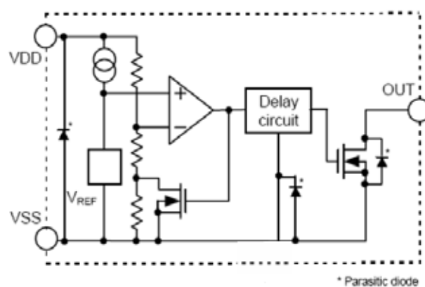
OPEN DRAIN (EC9518C)
