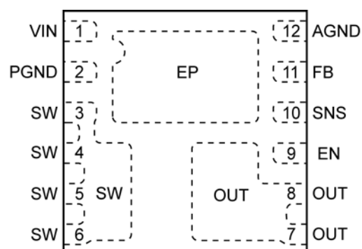
12-Pin 3mm x 3mm MLF ® (HL) Adjustable Output
