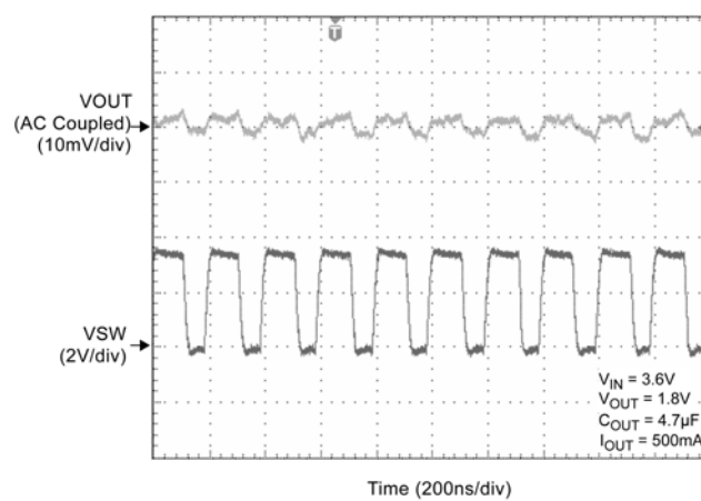
Switching Waveform
