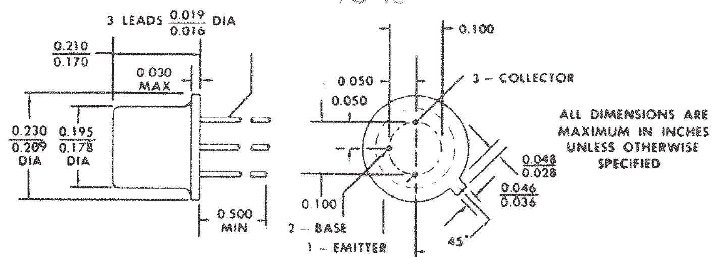
TO-18
