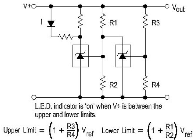
Fig 14. Voltage monitor
