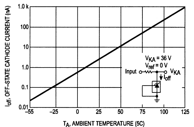
Fig 24. Off state cathode current versus ambient temperature
