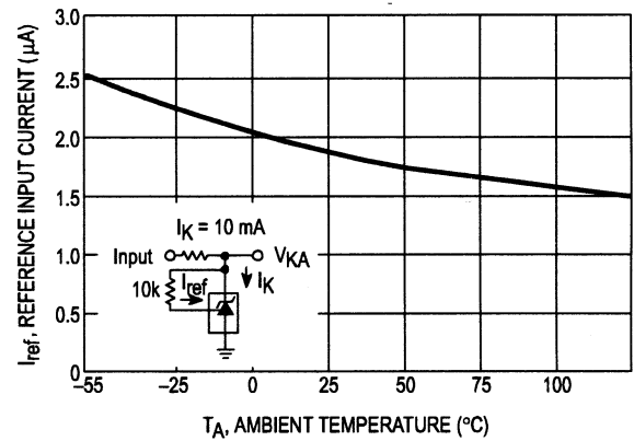
Fig 22. Reference input current versus ambient temperature
