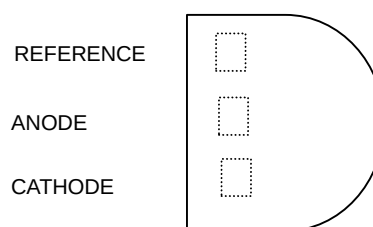
TO-92 TOP VIEW
