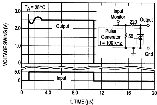
Fig 29. Pulse response
