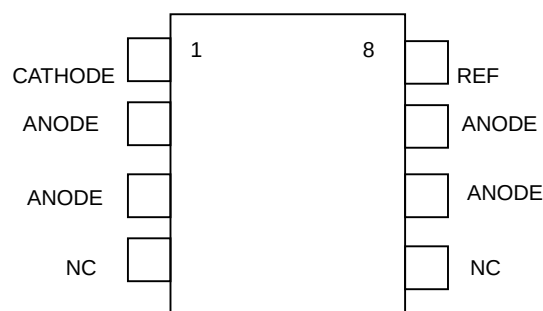
SOP-8 TOP VIEW
