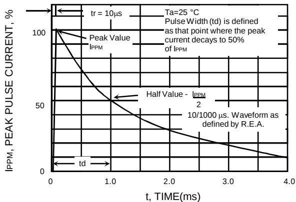
FIG.3 - PULSE WAVEFORM
