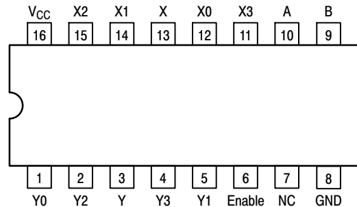
Figure 5. MC74HC4852A 16-Lead Pinout (Top View)
