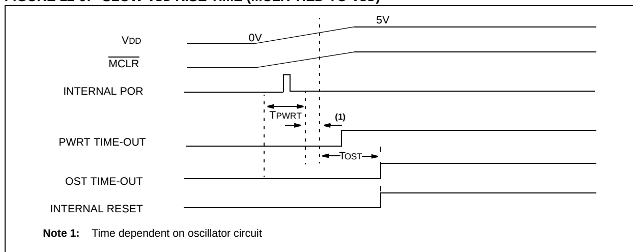
FIGURE 12-9: SLOW V_{DD} RISE TIME ( \overline{\text{MCLR}} TIED TO V_{DD} )
