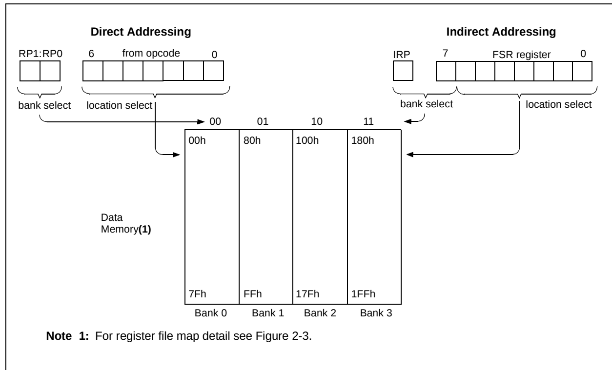
FIGURE 2-5: DIRECT/INDIRECT ADDRESSING
