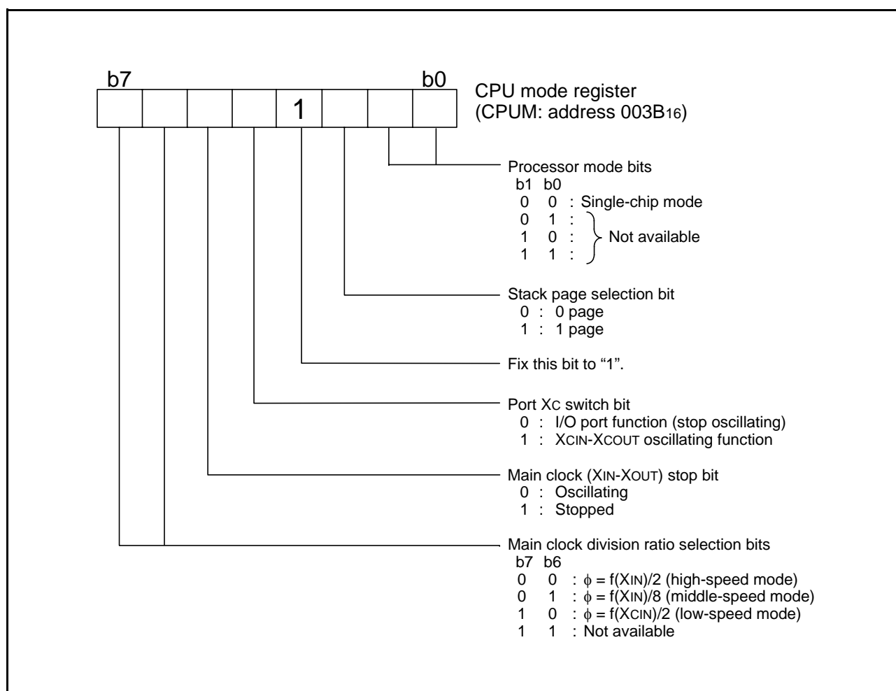
Fig. 9 Structure of CPU mode register
