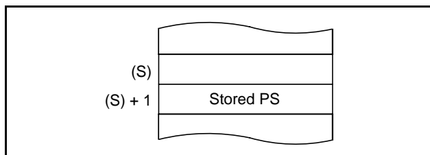
Fig. 102 Stack memory contents after PHP instruction execution
