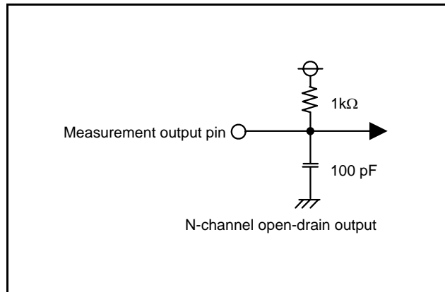
Fig. 115 Circuit for measuring output switching characteristics (2)
