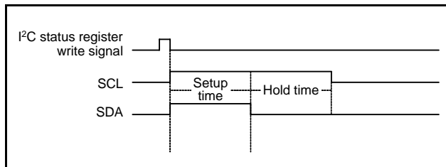
Fig. 66 START condition generating timing diagram
