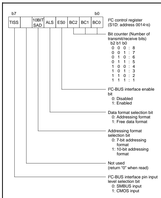
Fig. 63 Structure of I 2 C clock control register
