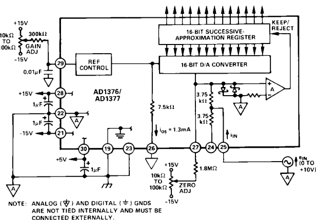
Figure 11. Analog and Power Connections for Unipolar 0 V to +10 V Input Range
