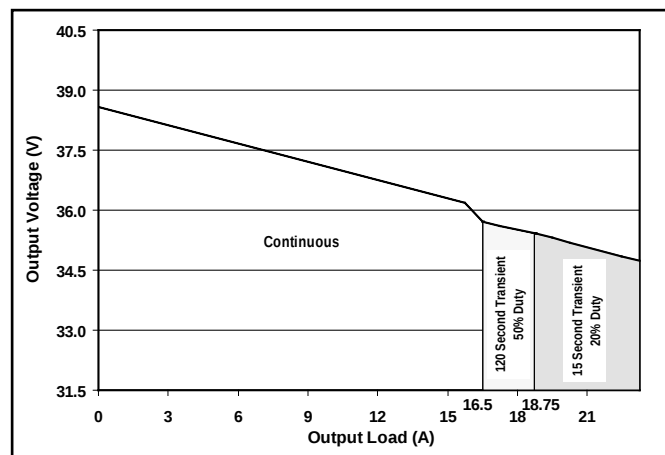
Figure 6: 36 V OUT droop characteristics.
