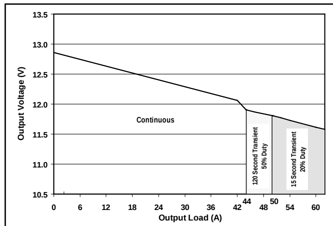
Figure 2: 12 V OUT droop characteristics.
