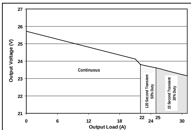
Figure 4: 24 V OUT droop characteristics.
