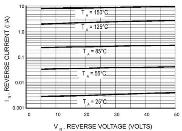
Figure 3. Leakage Current
