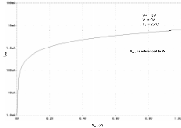
Current Sinking Versus V_{OUT}
