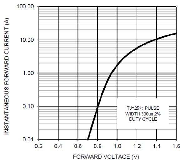
FIG. 2-TYPICAL FORWARD CHARACTERISTICS
