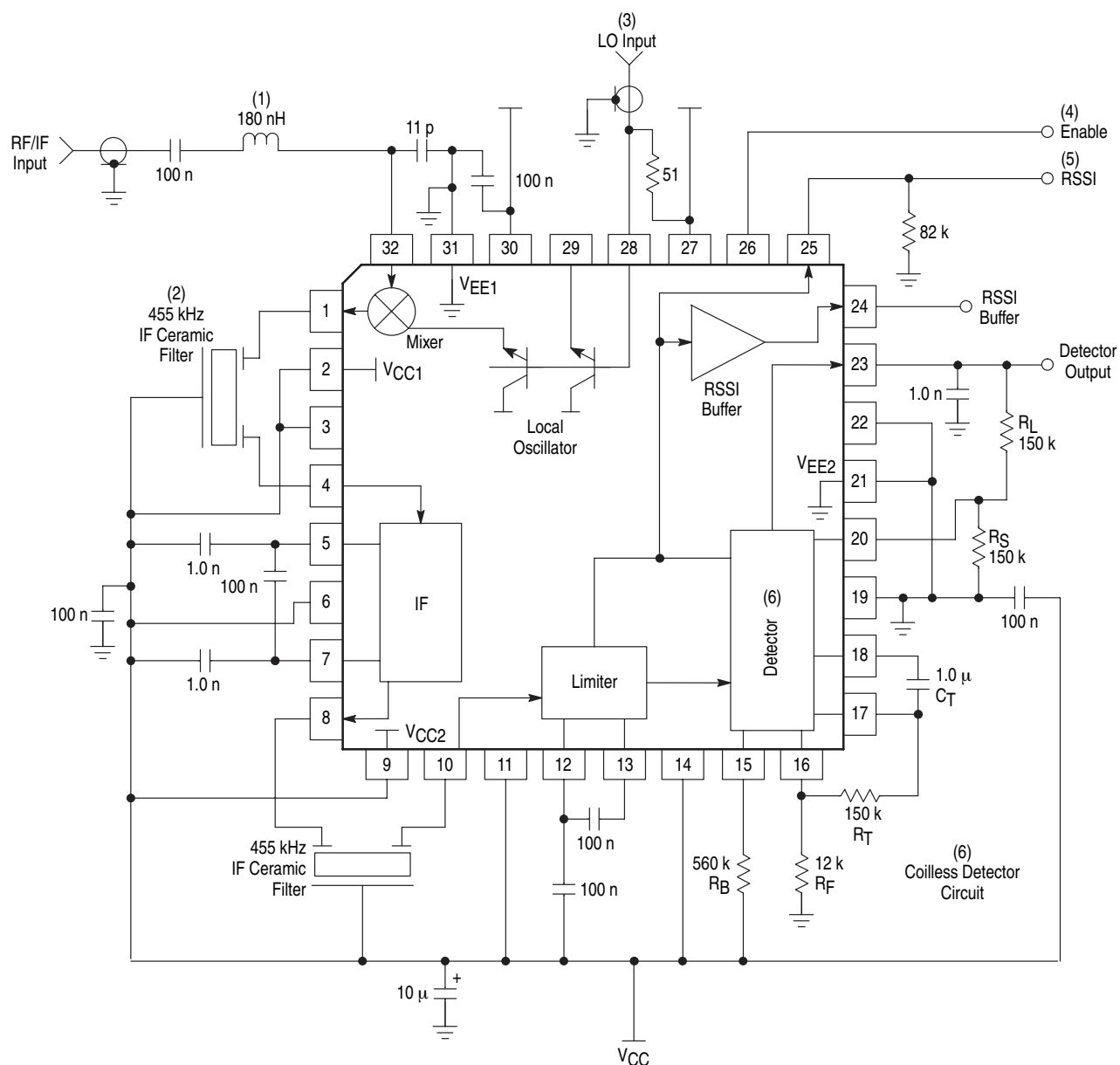
Figure 15. Application Circuit
