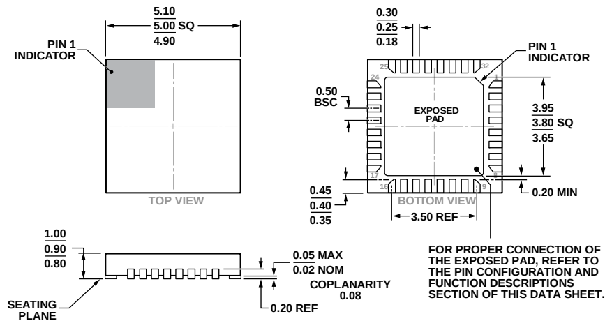
Figure 18. 32-Lead Lead Frame Chip Scale Package [LFCSP] 5 mm × 5 mm Body and 0.90 mm Package Height (HCP-32-3)
