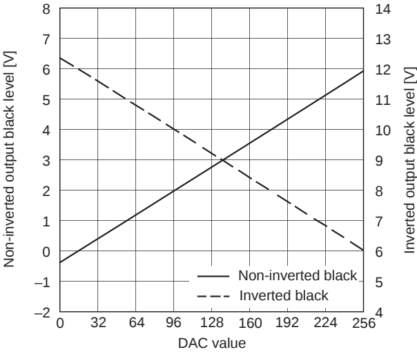
USER-BRIGHT adjustment characteristics
