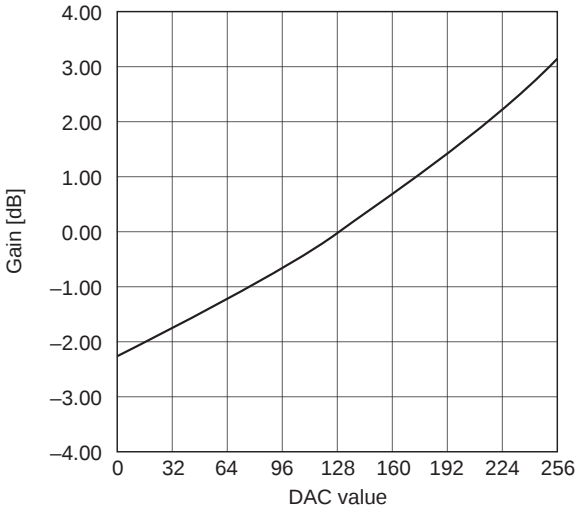
SUB-CONTRAST adjustment characteristics ( \gamma_1 = \gamma_2 = 0 )
