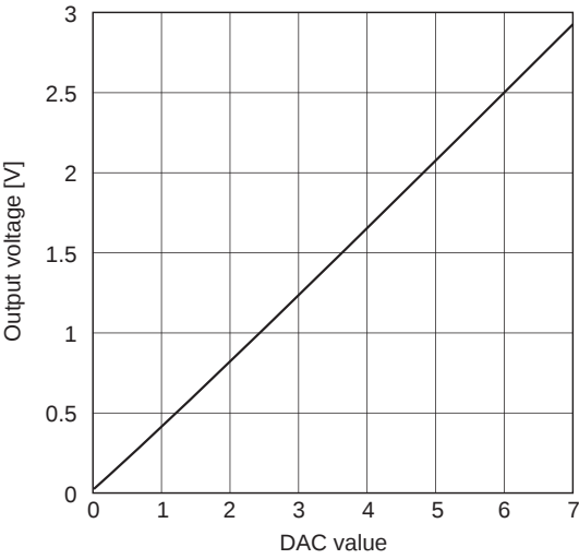
DA OUT output adjustment characteristics
