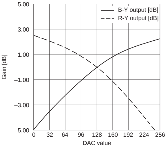
Color difference balance adjustment
