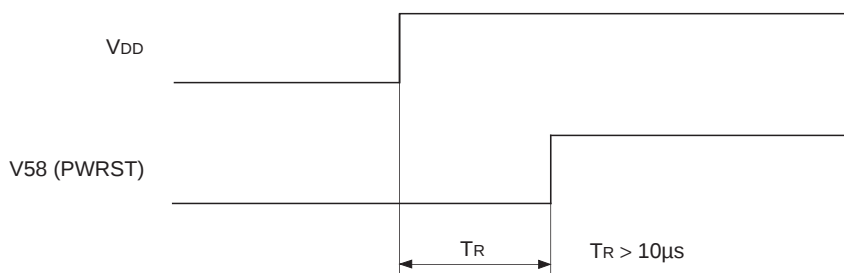
Fig. 1-1. System reset
