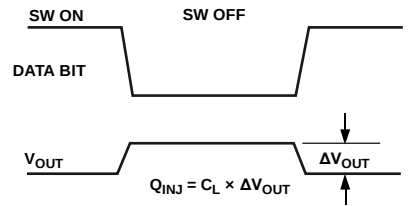
Figure 29. Charge Injection
