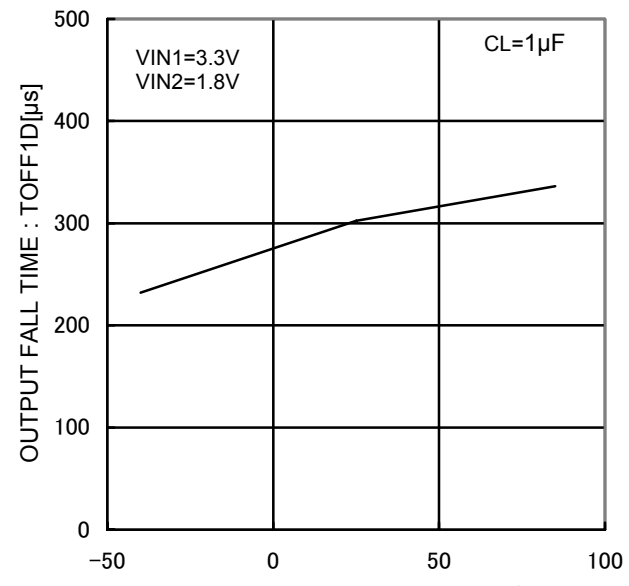
Figure 23. Output fall time1 DISC
