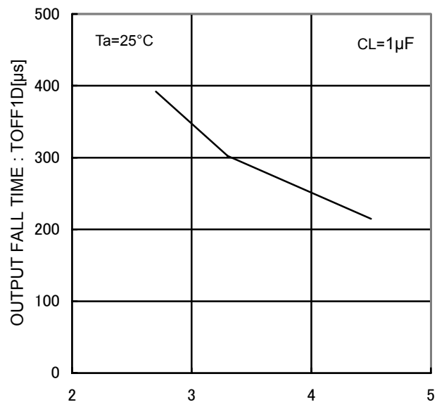
Figure 22. Output fall time1DISC
