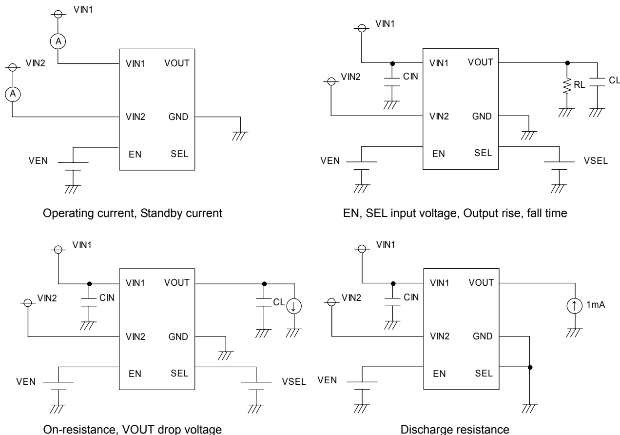
Figure 5. Measurement circuit
