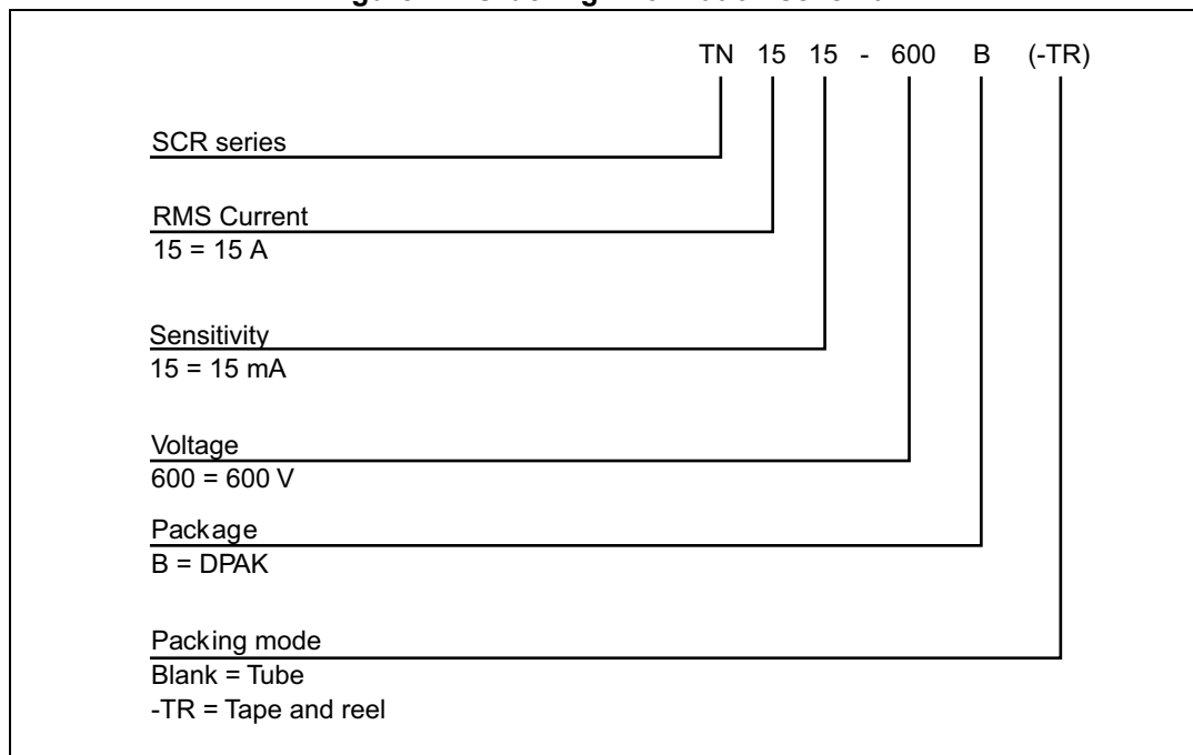
Figure 12. Ordering information schema
