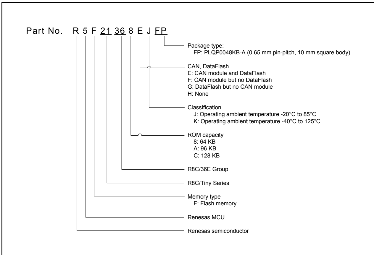
Figure 1.1 Part Number, Memory Size, and Package of R8C/36E Group
