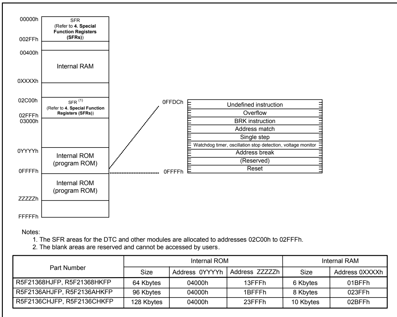
Figure 3.4 Memory Map of R8C/36H Group
