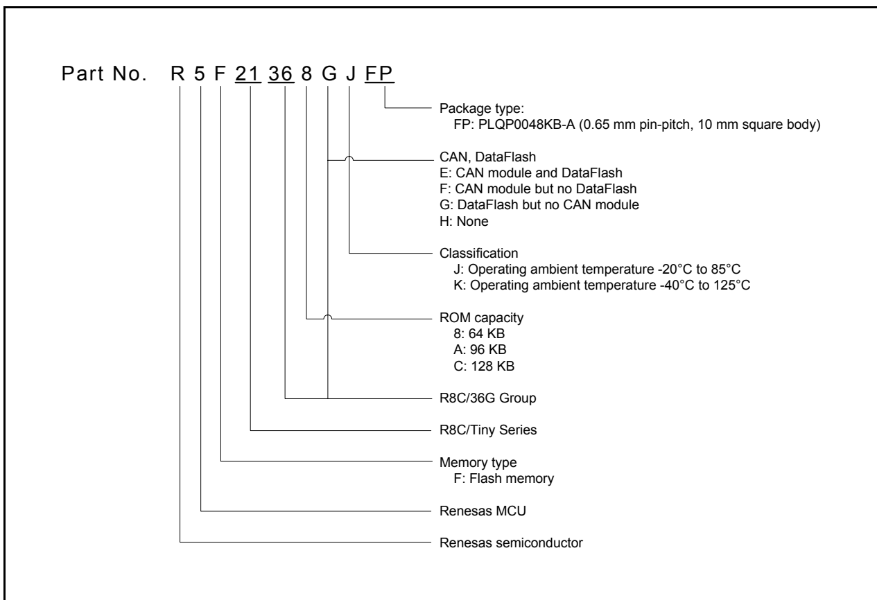
Figure 1.3 Part Number, Memory Size, and Package of R8C/36G Group
