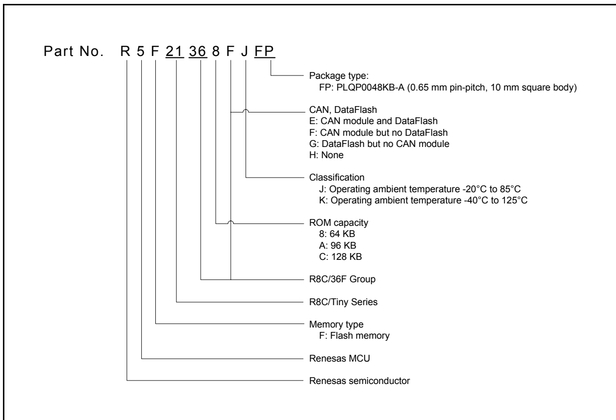
Figure 1.2 Part Number, Memory Size, and Package of R8C/36F Group
