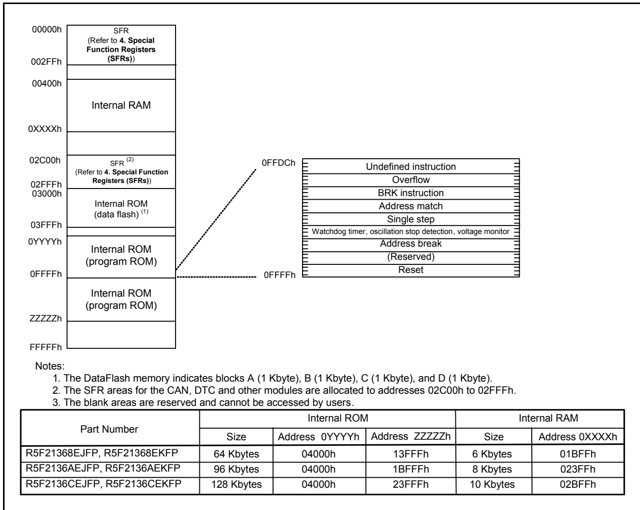
Figure 3.1 Memory Map of R8C/36E Group
