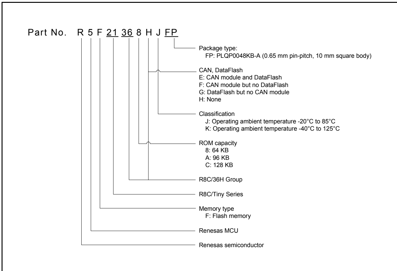
Figure 1.4 Part Number, Memory Size, and Package of R8C/36H Group
