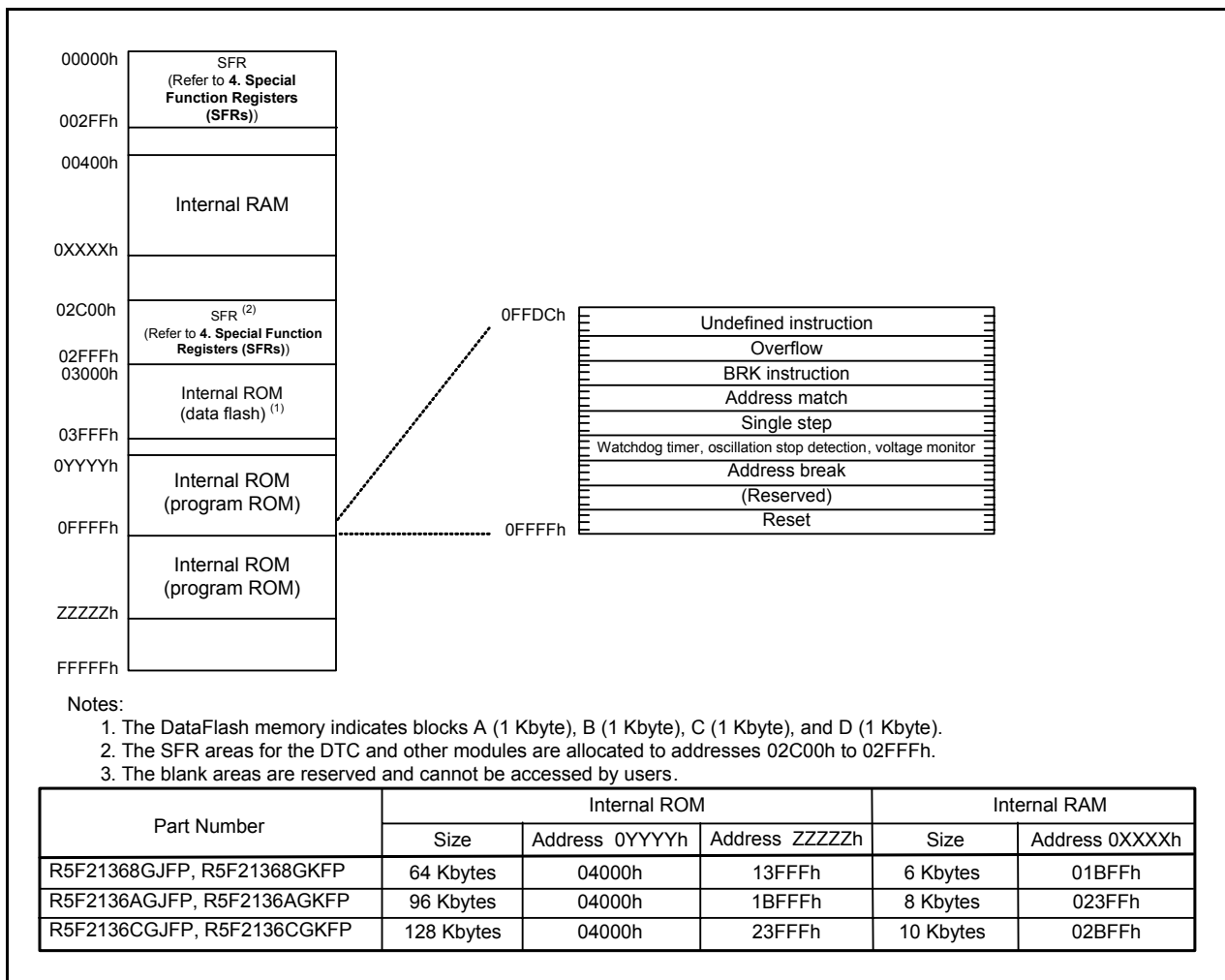
Figure 3.3 Memory Map of R8C/36G Group
