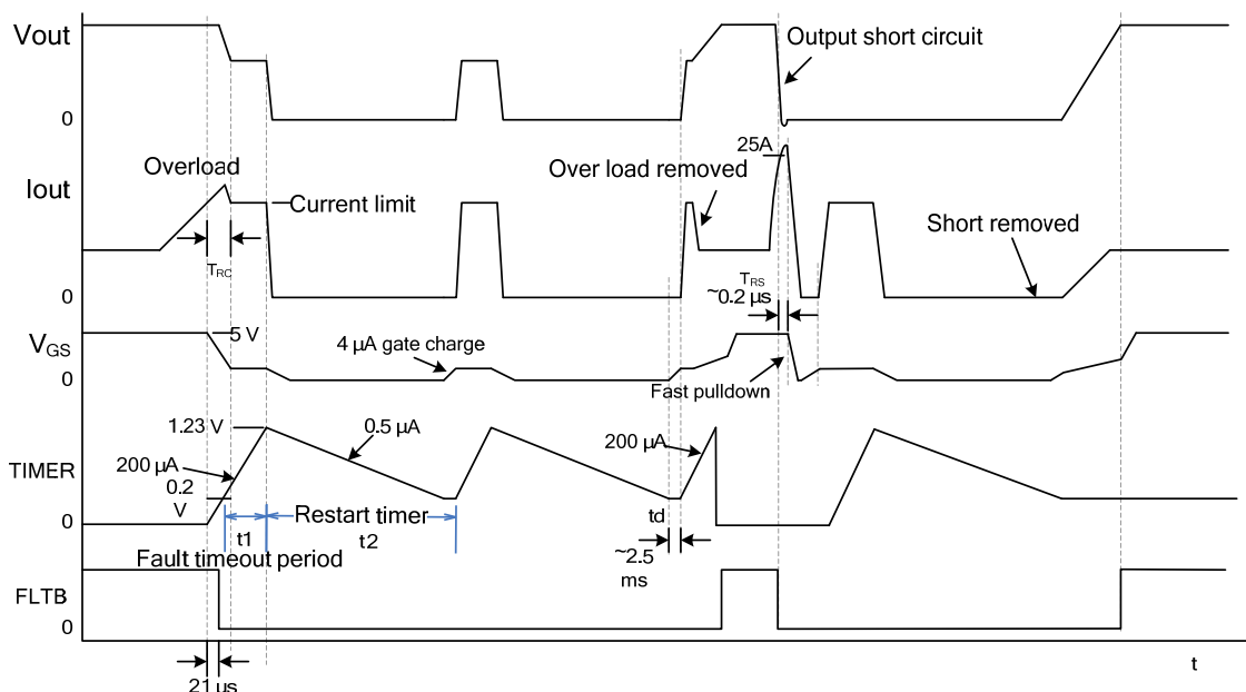
Figure 3—Over-current protection (auto-retry mode, AUTO = High)
