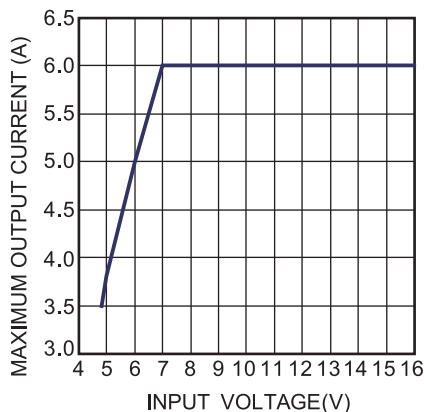
Maximum Continuous Current vs. Input Voltage
