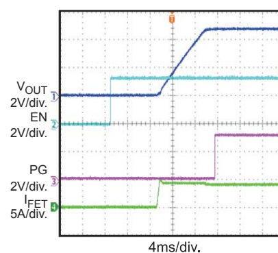
Start-Up through EN I OUT =3.8A
