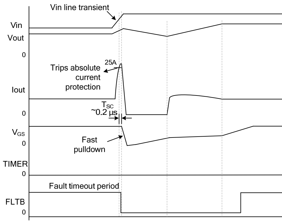
Figure 4—Input voltage line transient response
