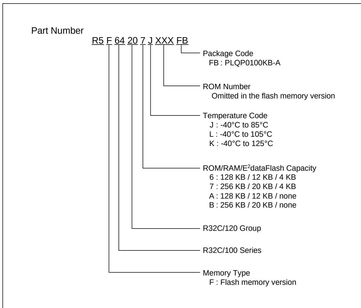
Figure 1.1 Part Numbering
