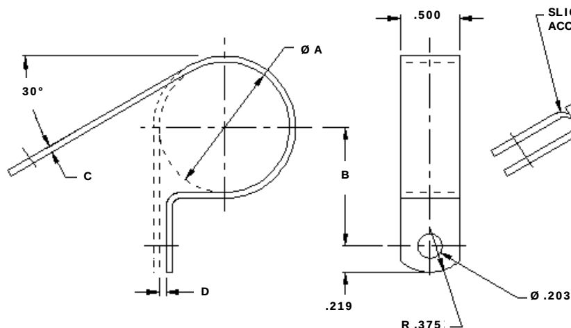
PLAIN CLAMP
