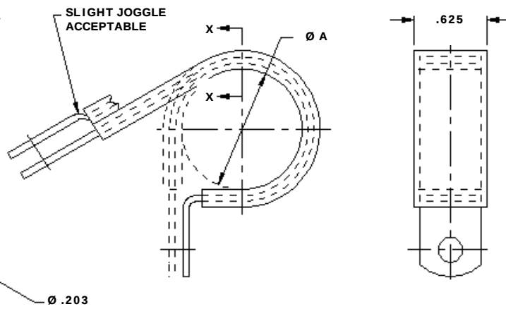
CUSHIONED CLAMP
