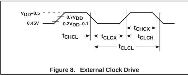
Figure 8. External Clock Drive
