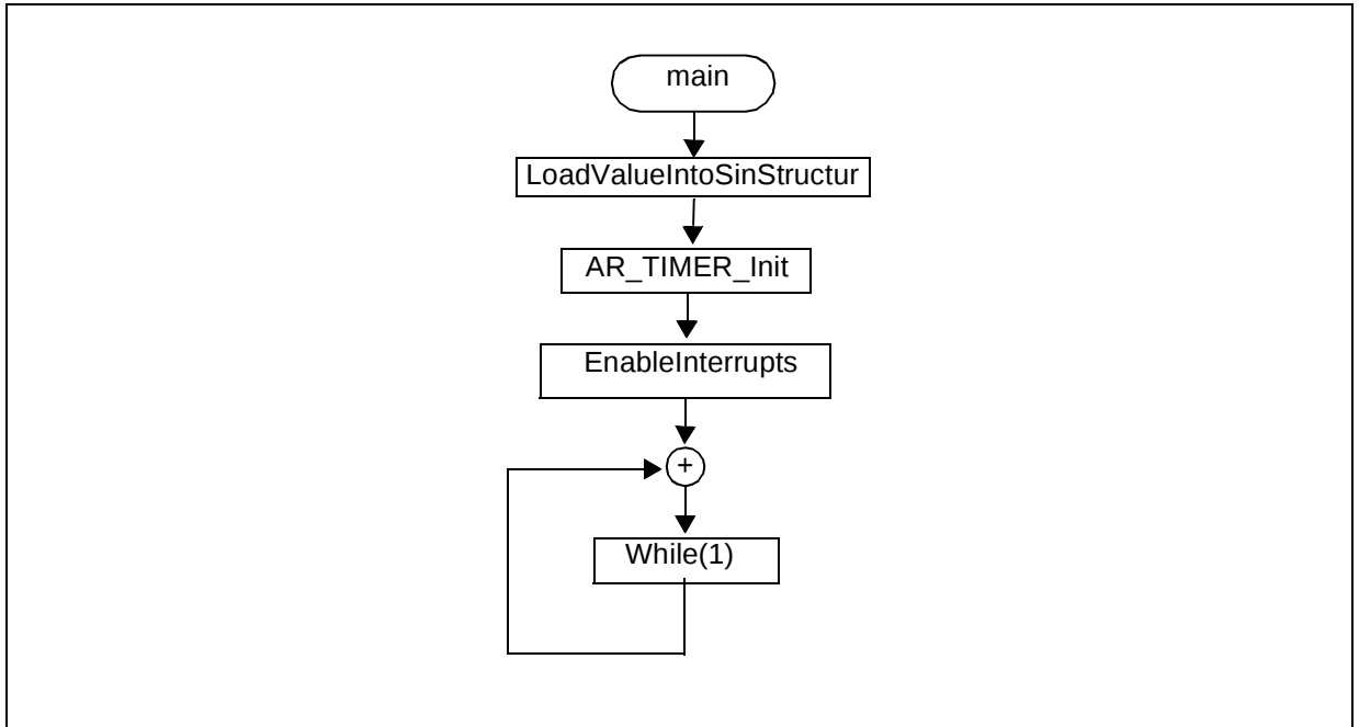
Figure 6. Main routine
