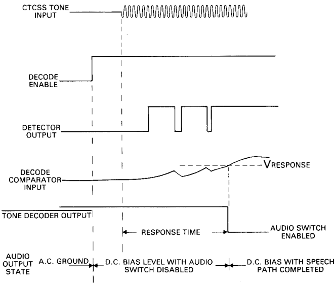
Fig. 4 Decoder Response Sequence
