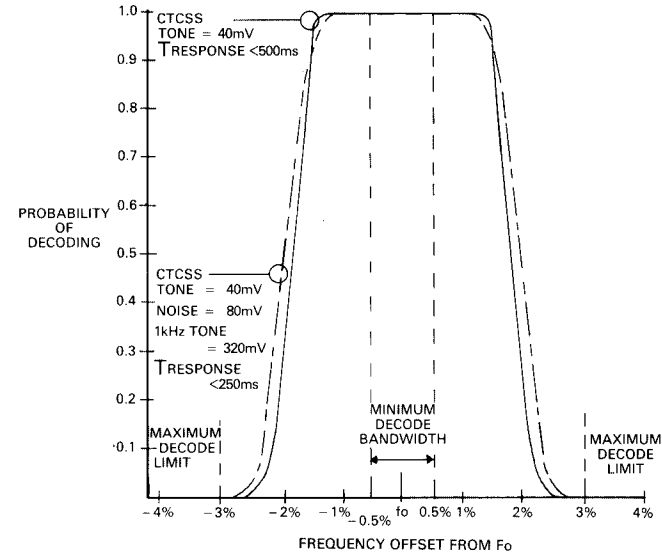
Fig. 6 Decoder Probability Curves
