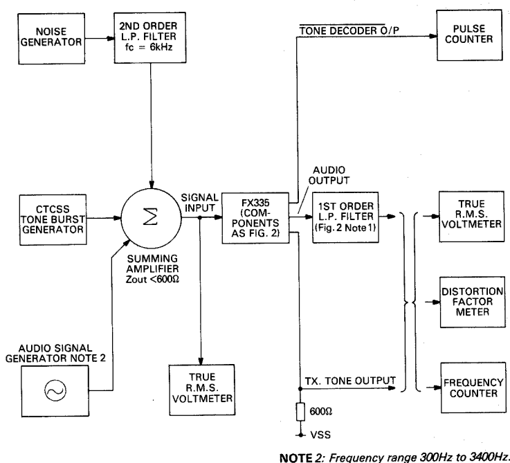
Fig. 3 Test Set up
