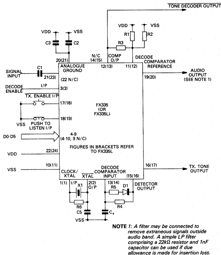
Fig. 2 External Component Connections
