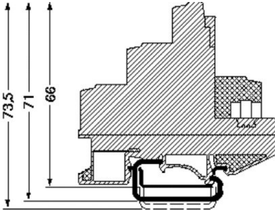
Dimensioned drawing
