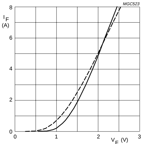
BYD33U and V Solid line: T_j = 25\text{ }^{\circ}\text{C} . Dotted line: T_j = 175\text{ }^{\circ}\text{C} .
