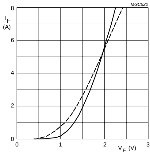
BYD33D to M Solid line: T_j = 25\text{ }^{\circ}\text{C} . Dotted line: T_j = 175\text{ }^{\circ}\text{C} .
