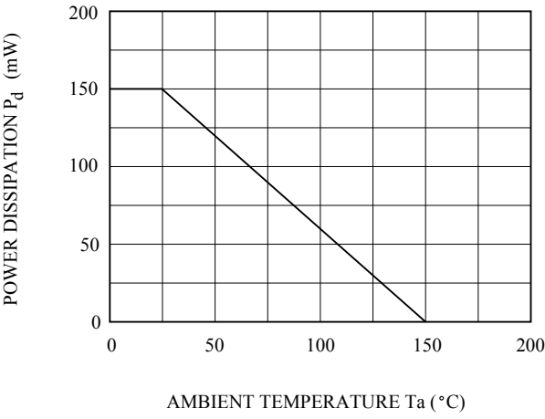
P_d - T_a
