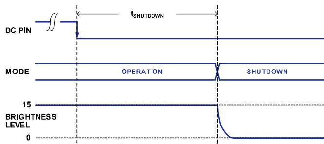
Figure 3. Shutdown Timing
