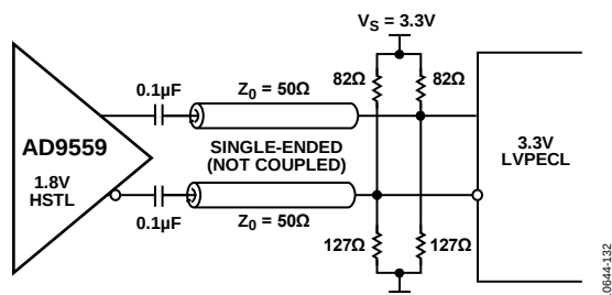
Figure 31. Interfacing the HSTL Driver to a 3.3 V LVPECL Input (This method incorporates impedance matching and dc-biasing for bipolar LVPECL receivers. If the receiver is self-biased, the termination scheme shown in Figure 29 is recommended.)
