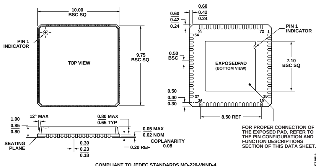
Figure 57. 72-Lead Lead Frame Chip Scale Package [LFCSP_VQ] 10 mm × 10 mm Body, Very Thin Quad (CP-72-4)
