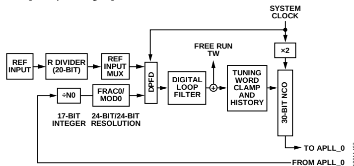
Figure 35. DPLL_0 Core
