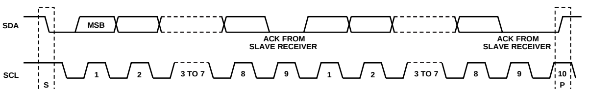
Figure 53. Acknowledge Bit
