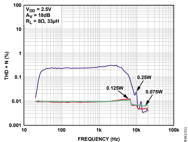
Figure 11. THD + N vs. Frequency, V_{DD} = 2.5V , R_L = 8\Omega , A_V = 18dB
