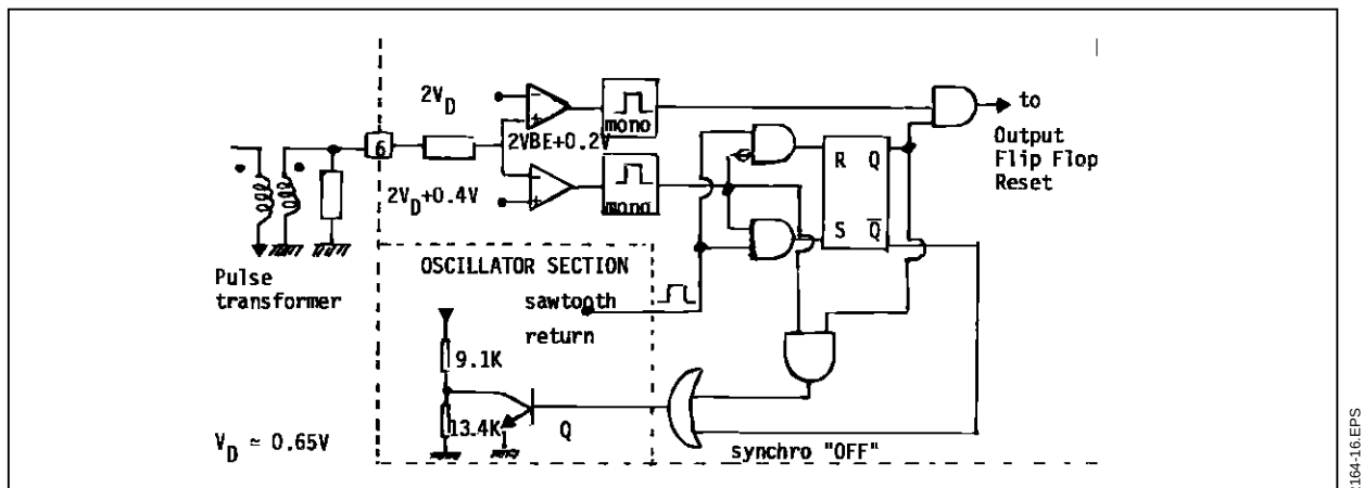
Figure 12 : Synchronization Pulse Shaper and Synchronization
