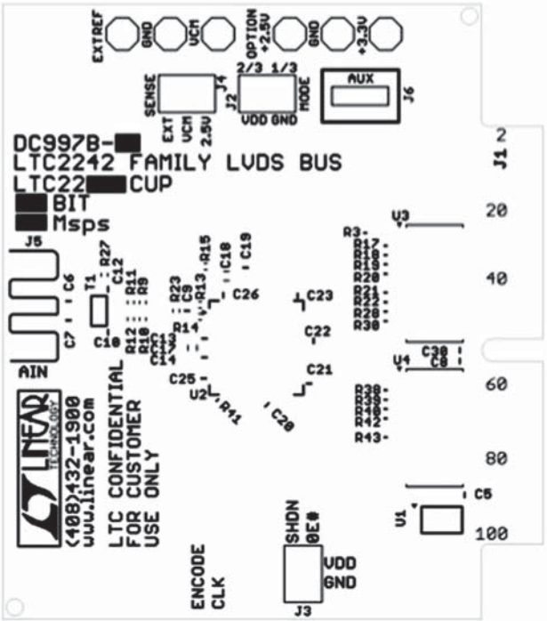
Silkscreen Top
