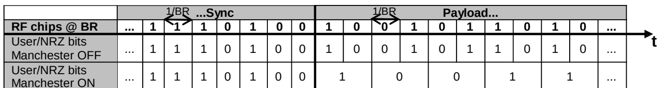
Figure 35. Manchester Encoding/Decoding
