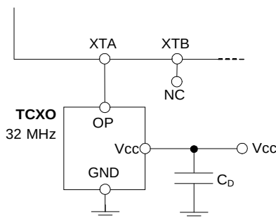
Figure 5. TCXO Connection
