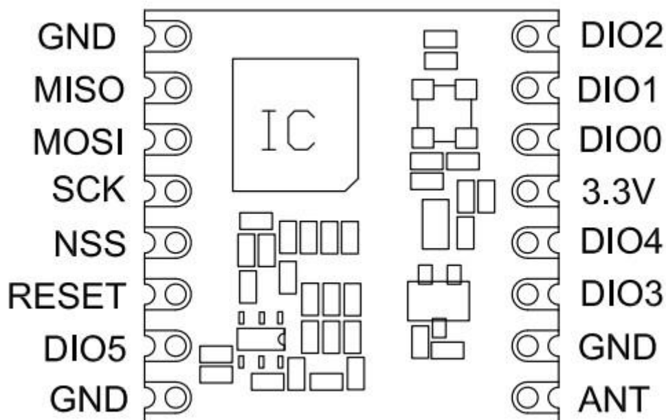
Figure 3. Marking Diagram
