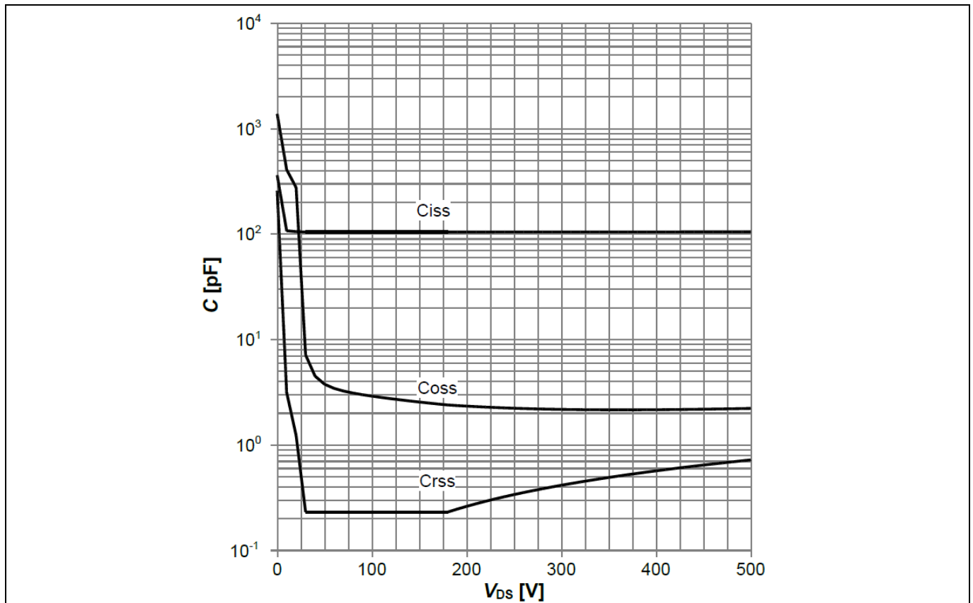
Figure 35 Typical CoolMOS™ capacitances of ICE5QR4780AZ ( C=f(V_{DS}); V_{GS}=0 V; f=250 kHz)
