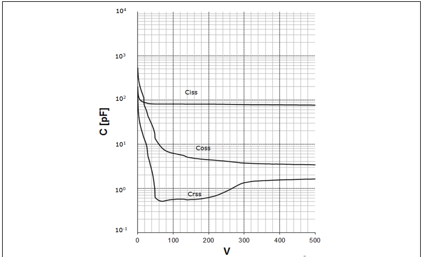
Figure 34 Typical CoolMOS™ capacitances of ICE5QR4770Ax ( C=f(V_{DS}); V_{GS}=0 V; f=1 MHz)
