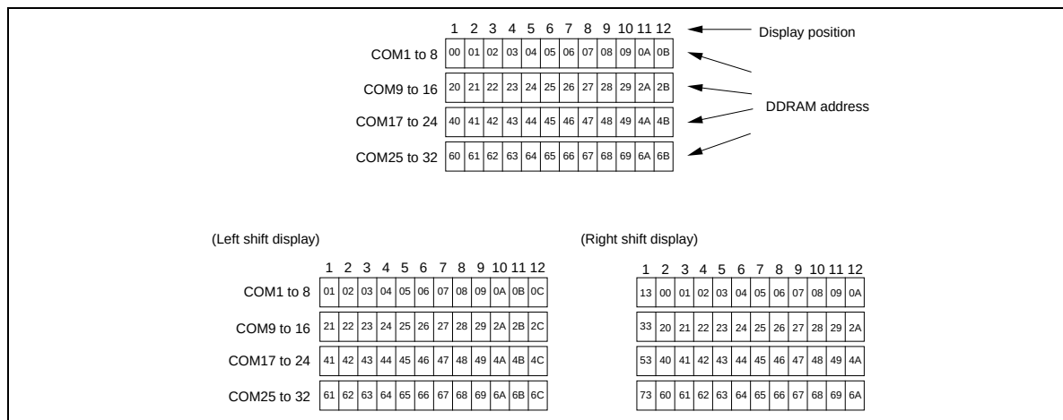
Figure 8 4-Line Display
