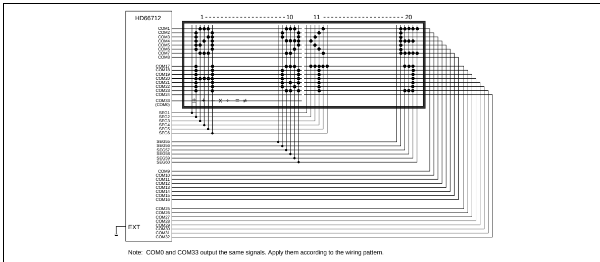
Figure 28 20 × 2-Line + 60 Segment Display (6-Dot Font, 1/33 Duty)
