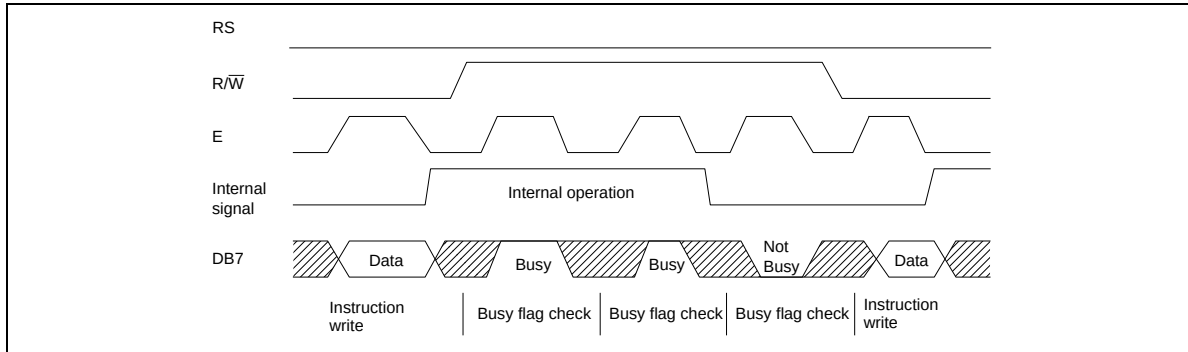
Figure 18 Example of 8-Bit Data Transfer Timing Sequence
