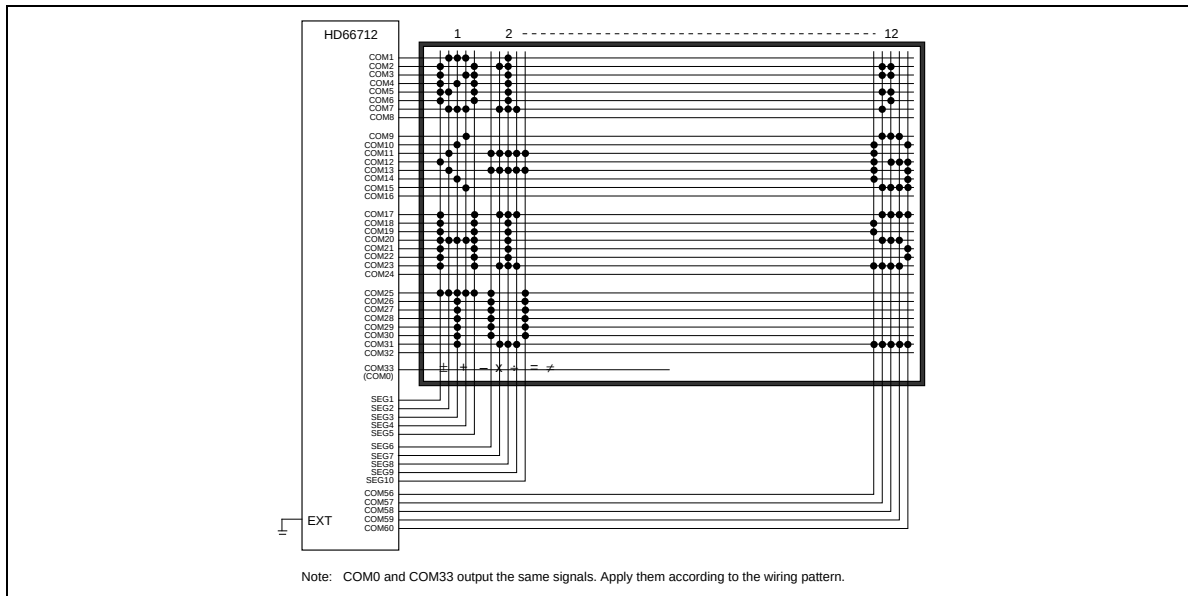
Figure 27 12 × 4-Line + 60 Segment Display (5-Dot Font, 1/33 Duty)
