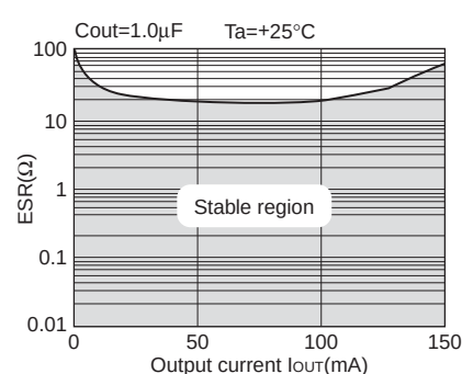
Fig. 32 BH□□LB1WHFV/WG Stable operating region characteristics (Example)
