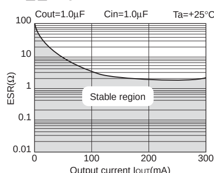
Fig. 34 BH□□MA3WHFV Stable operating region characteristics (Example)
