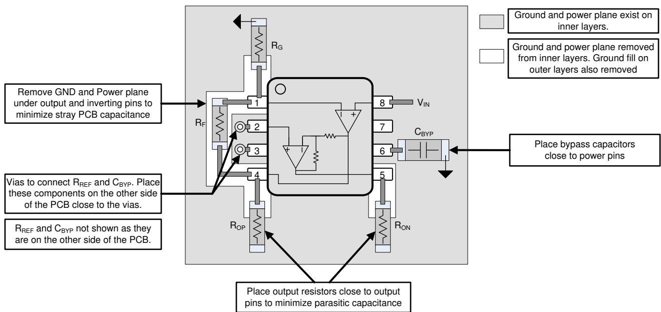
图 10-2. Layout Recommendations
