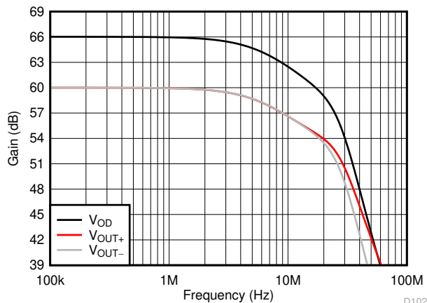
图 8-8. Small-Signal Bandwidth
