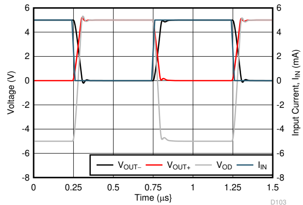
图 8-9. Large-Signal Transient Response
