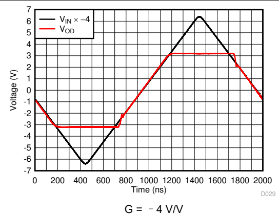
图 6-34. Output Overdrive Recovery
