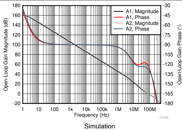
图 6-3. Open-Loop Gain And Phase vs Frequency
