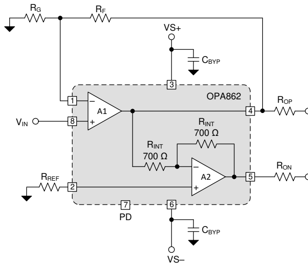
图 10-1. Representative Schematic for Layout in
