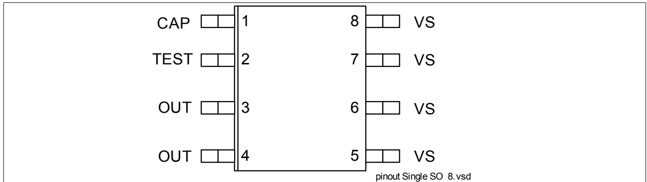
Figure 3 Pin Configuration
