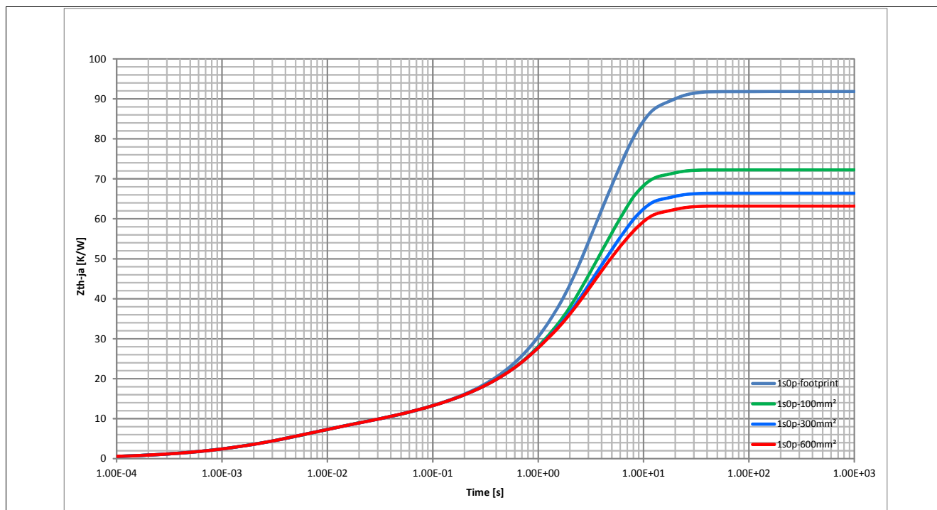
Figure 6 Typical Thermal Resistance for FR2 PCB
