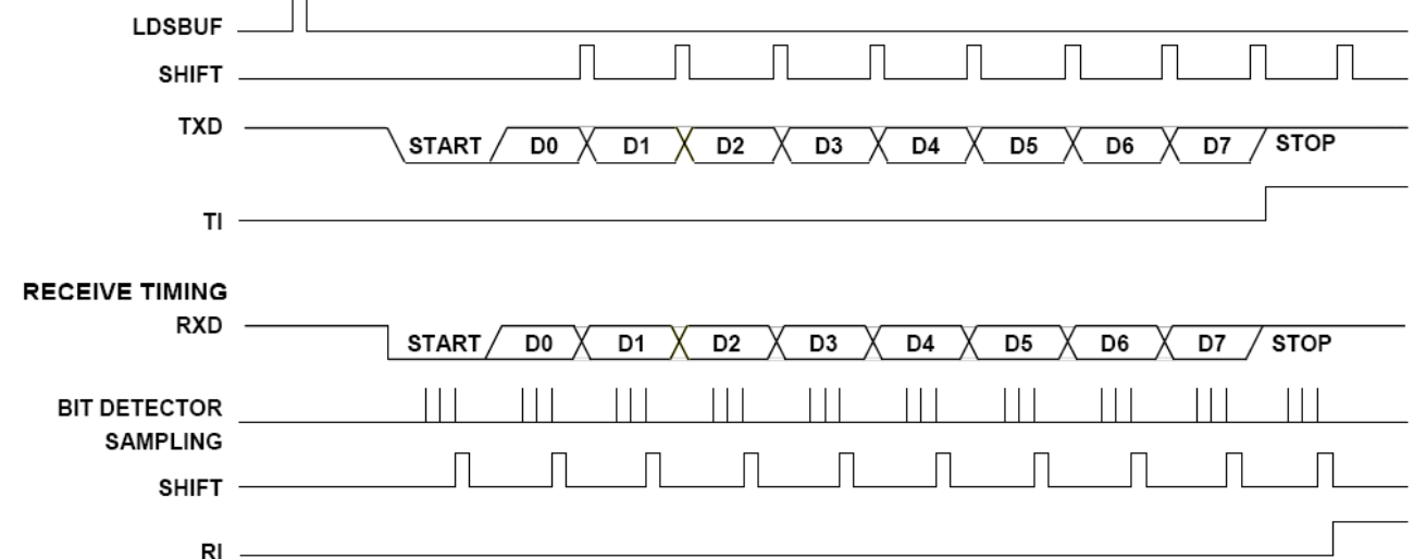
13-2. Serial Port Mode
