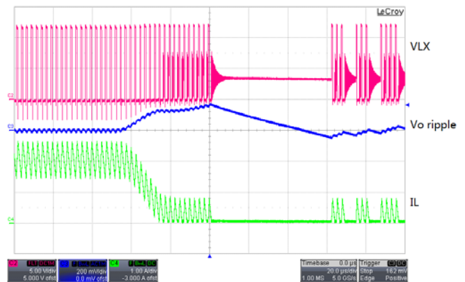
Figure 9. PWM to PEM Transition
