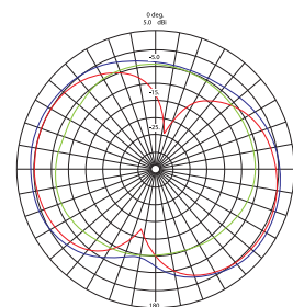
TYPICAL ELEVATION PATTERN
