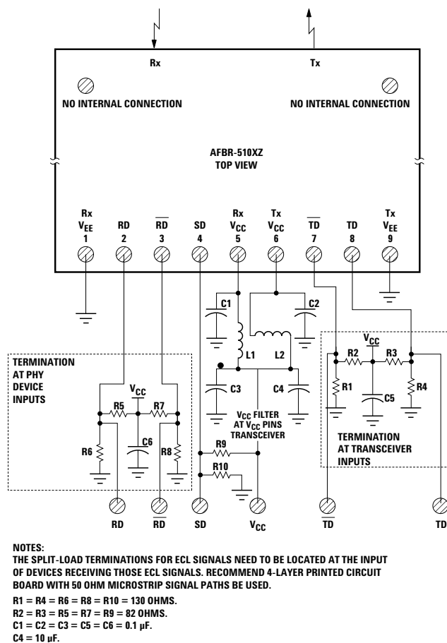
Figure 7. Recommended Decoupling and Termination Circuits
